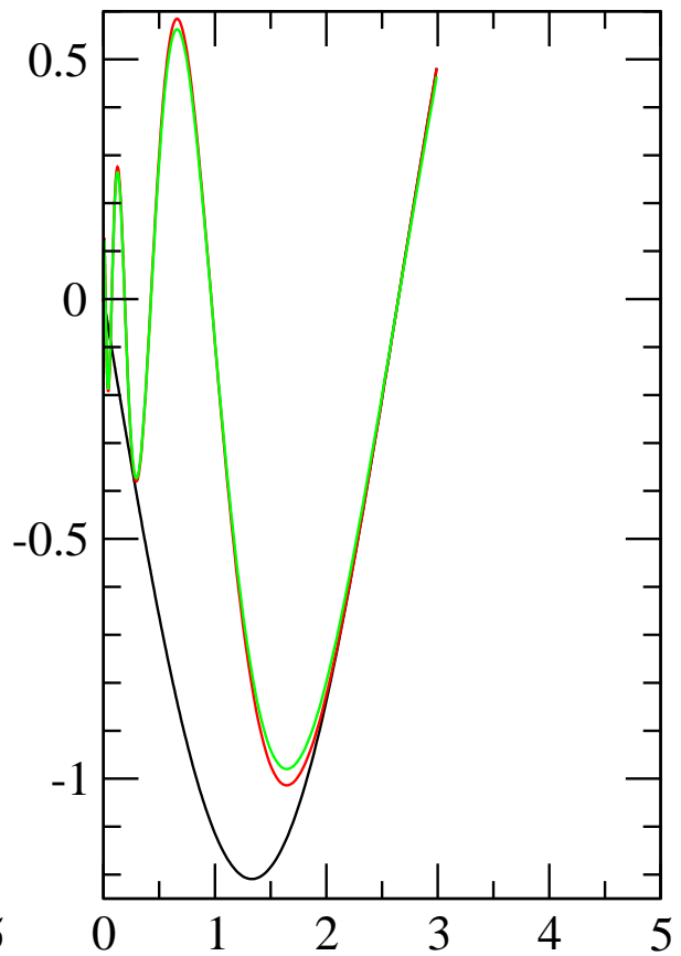
wfn8, l=0
