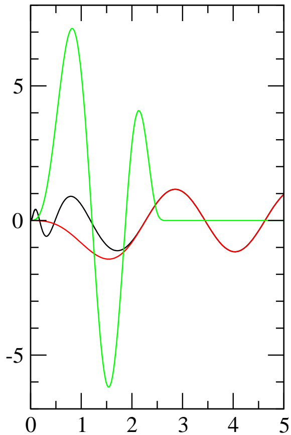
wfn7, l=2
