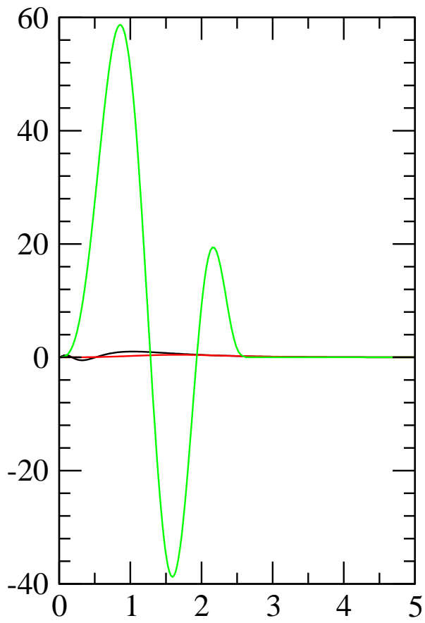
wfn5, l=2
