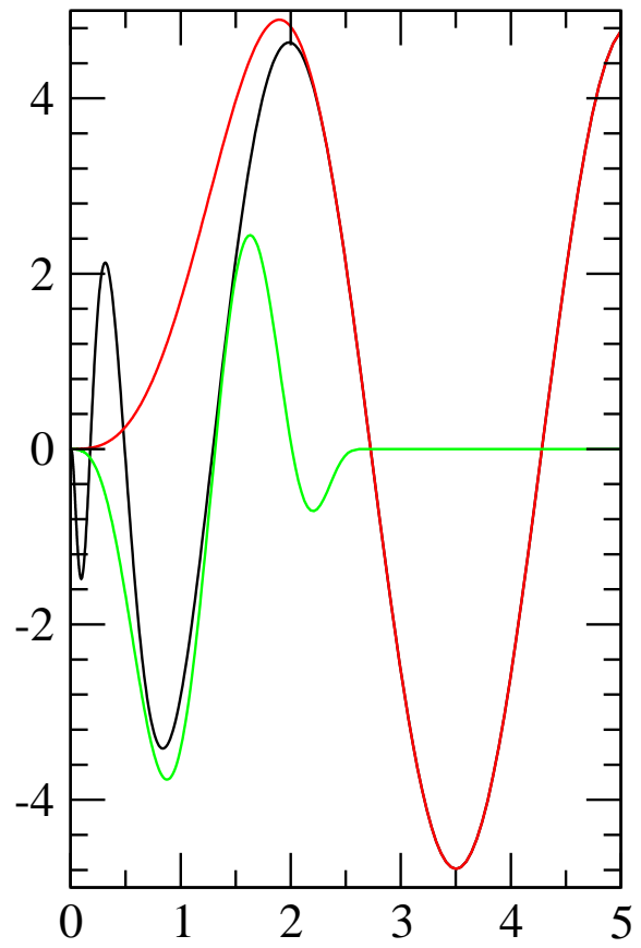
wfn8, l=0
