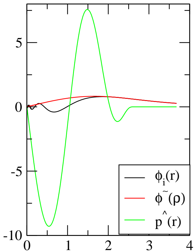
wfn3, l=1
