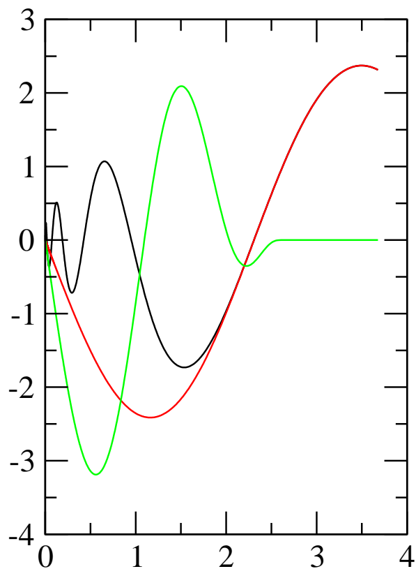
wfn4, l=4
