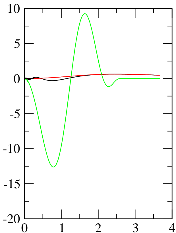
wfn3, l=1
