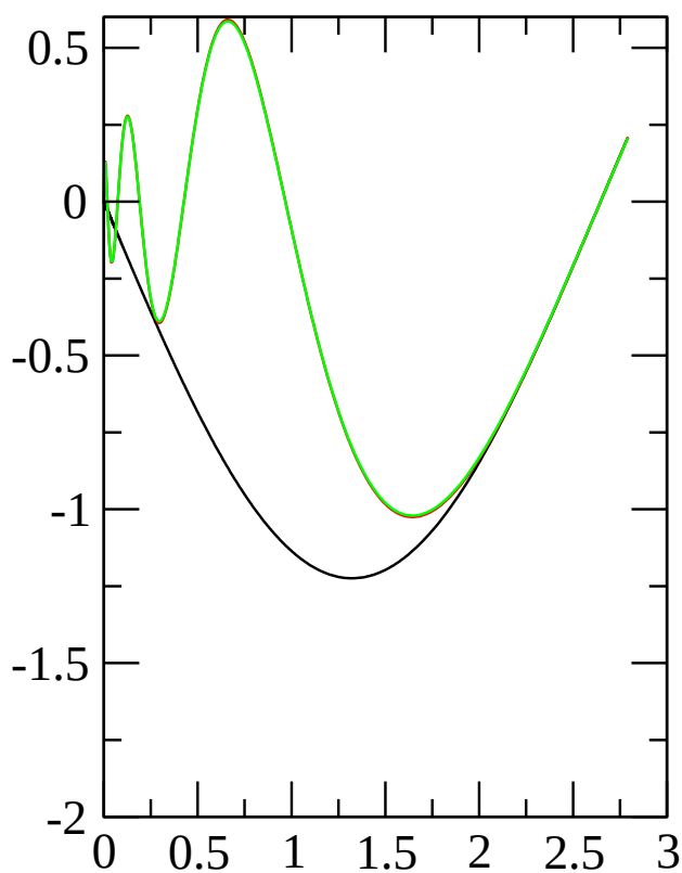
wfn7, l=0
