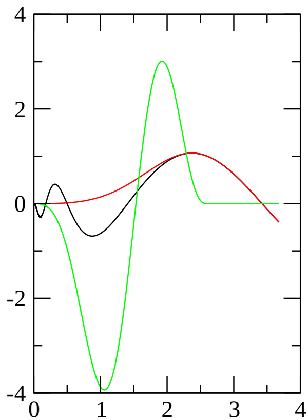
wfn8, l=1
