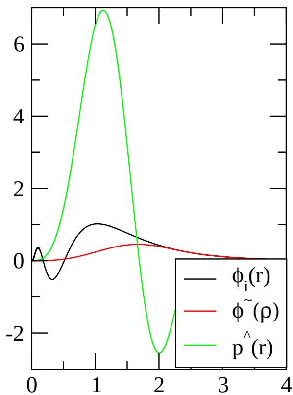
wfn7, l=0
