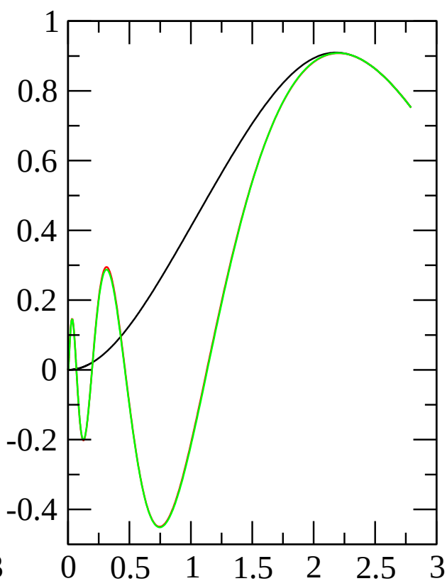
wfn8, l=1
