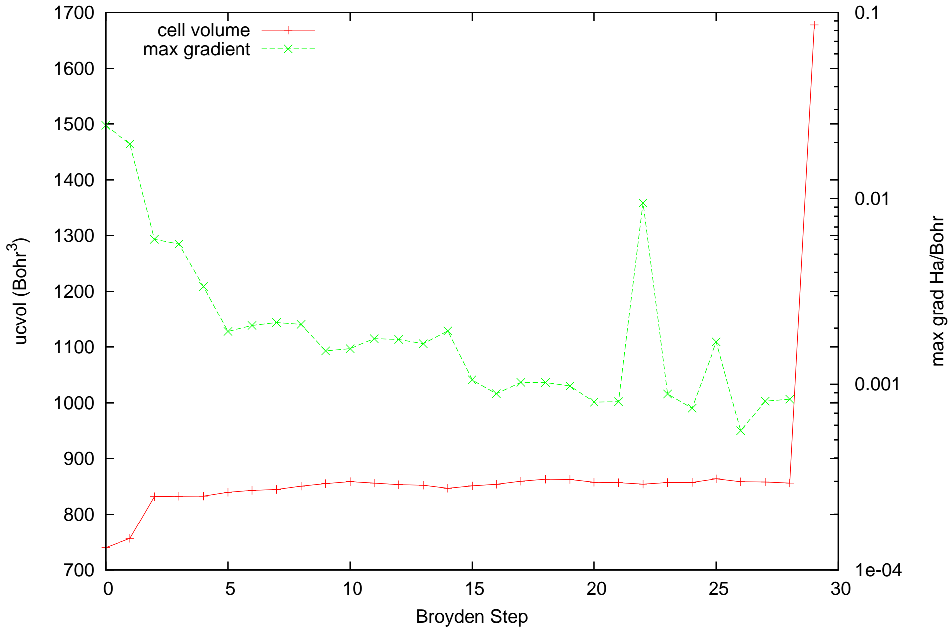
Structural Optimization: ionmov 2, optcell 1
